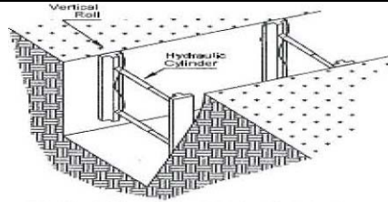
Vertical Aluminum Hydraulic Shoring (Spot Bracing)
